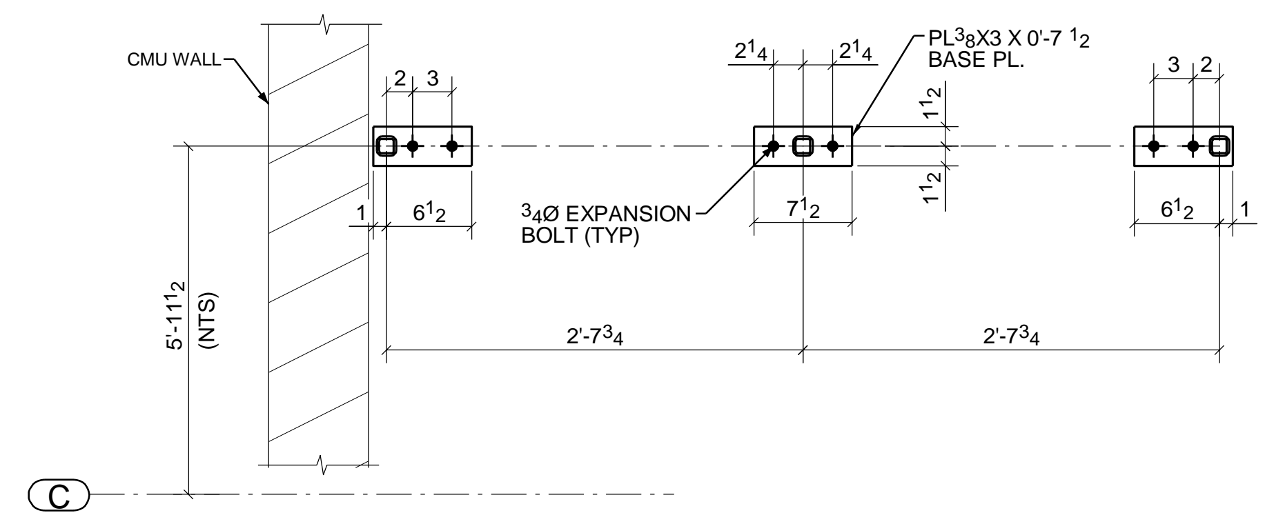
SECTION H - H
